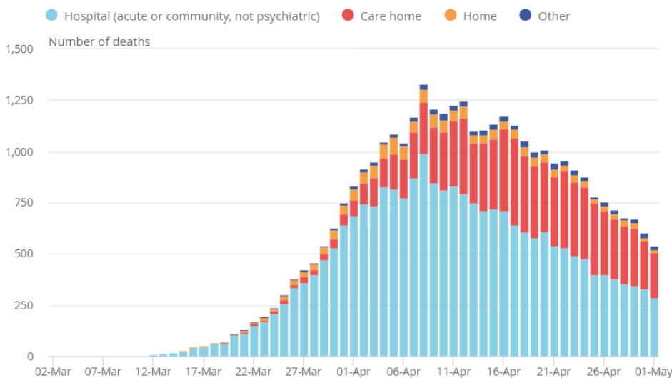
3 Number of deaths by actual date of death registered up to 9 May, by the place the death occurred and per day for England and Wales, 2020
